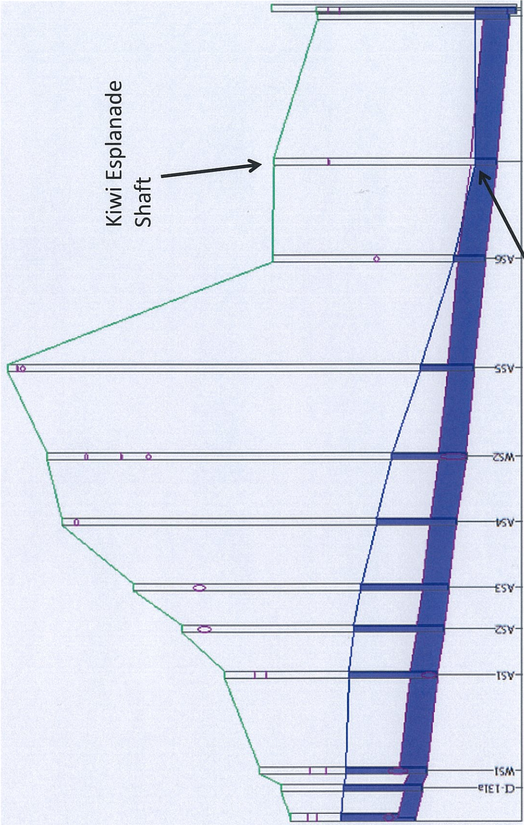
Figure1 – Pressure air release vent required at Kiwi Esplanade
